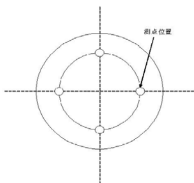
图4 圆形风口测点布置
